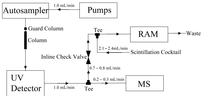
Fig. 2. Schematic diagram of a LC-MS system with a homogeneous in-line radioactivity flow detector.
