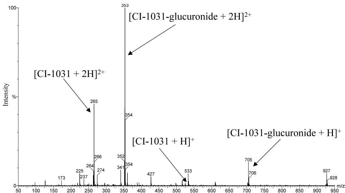
Fig. 5. LC-MS Spectrum of 0–4 h urine following a single 1 mg/kg intravenous bolus dose of [^{14}\text{C}] CI-1031 to male rats.
